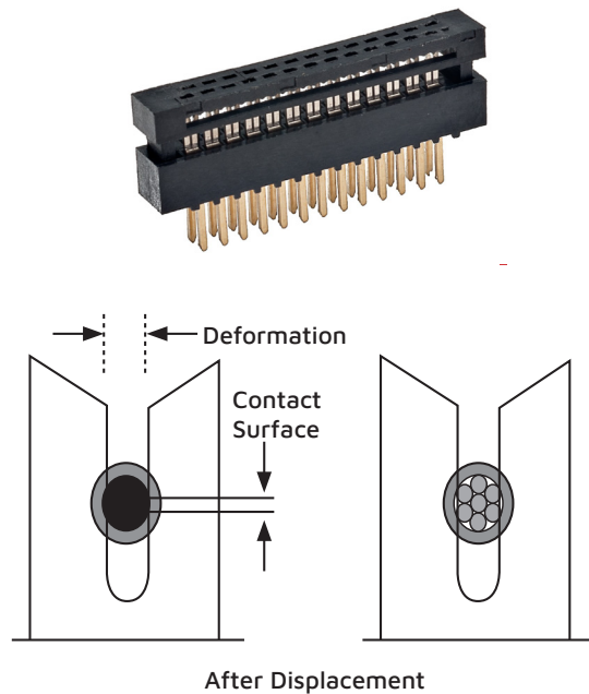
Figure 4: IDC connector, with cross-sectional views
